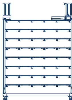
Innorack® Rat 3.5, dimensions and cage positions.
