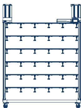
Innorack® IVC Tall Rat, dimensions and cage positions.
